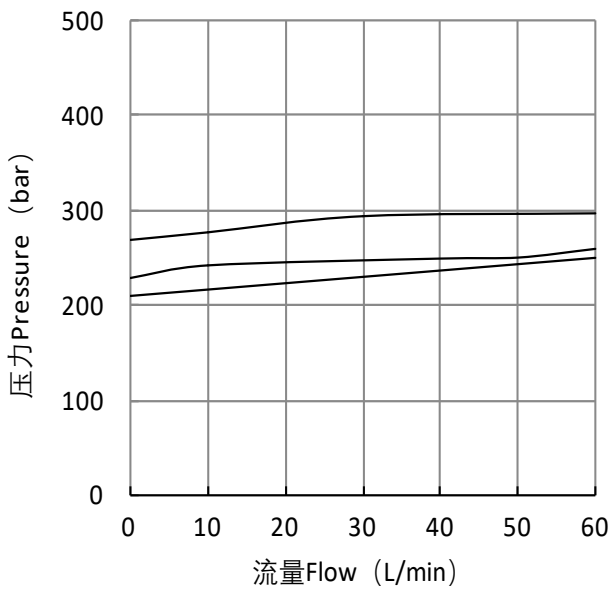
弹簧4=(211-280bar) Spring4= (211-280bar)
