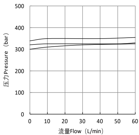
弹簧 6=(351-420bar) Spring 6=(351-420bar)
