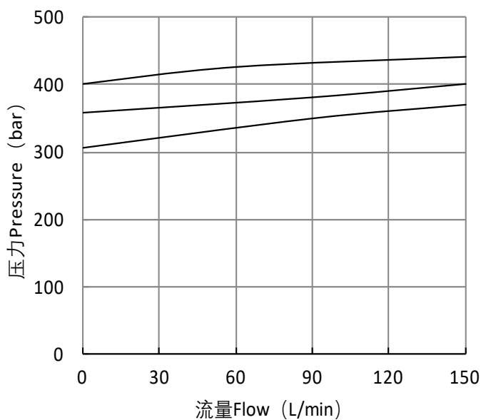
弹簧5=(321-400bar) Spring 5= (321-400bar)
